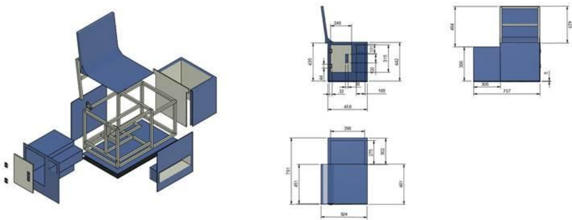
Fig. 6. Exploded view of the final design (left) and overall dimensions in mm (right).
